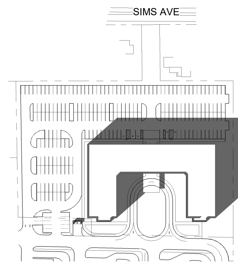
③ SPRING EQUINOX 3pm 1 : 1500
