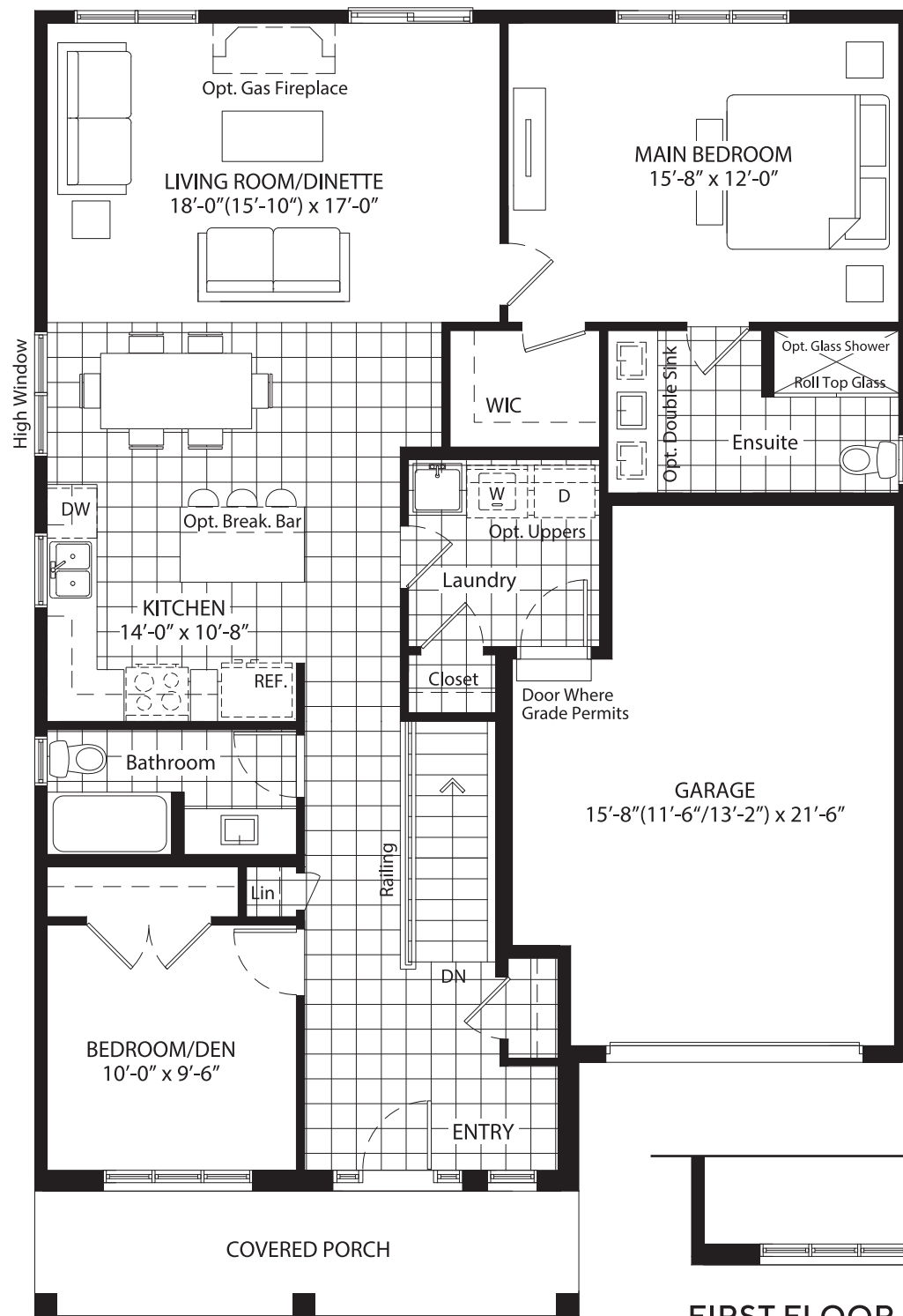
FIRST FLOOR ELEVATION B
